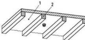
Example of subsections with a height of > 0.2 m and a ceiling section > 36 m²
