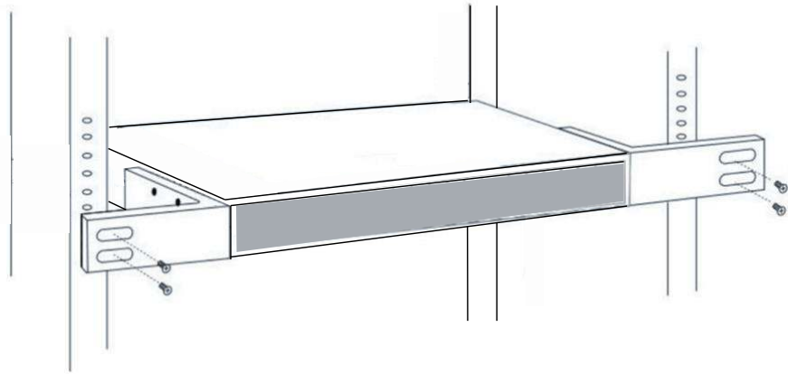
Rack Installation
