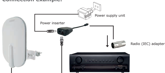
Connection example:
