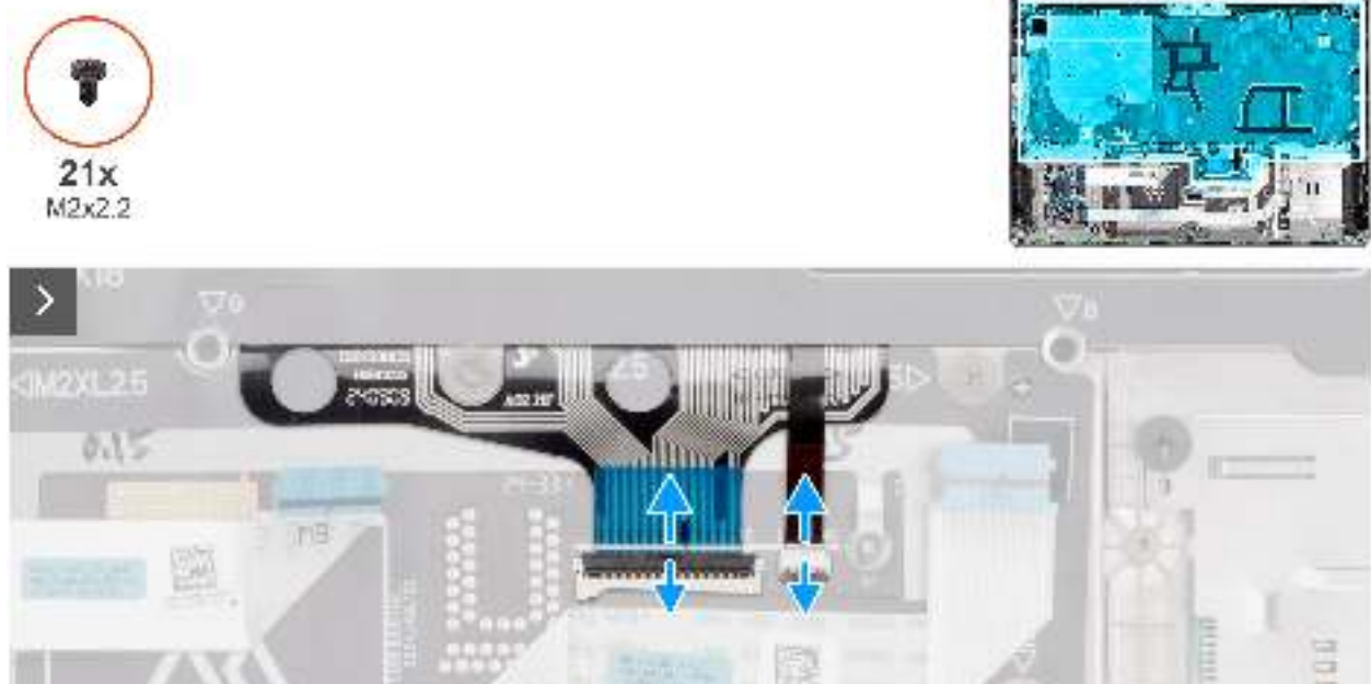
Abbildung 94. Removing the keyboard
