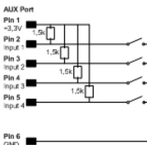
Abbildung 145: Examples: AUX Input on hardware model CS131 only, left side “pull-down”, right side “pull-up” configuration
