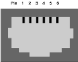
Abbildung 141: AUX-Port (Hardware Revision 1.1 = from Serial numbers 0121-1203, 0122-00198, 0123-00564 onwards) RJ11 6-pol
